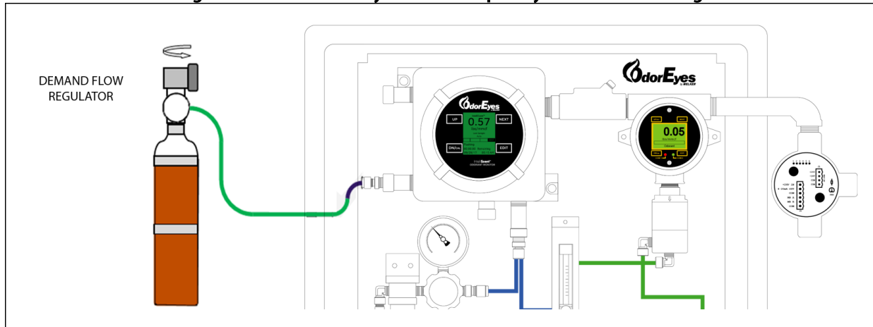
Figure 18: Calibration Cylinder – Temporary External Mounting
