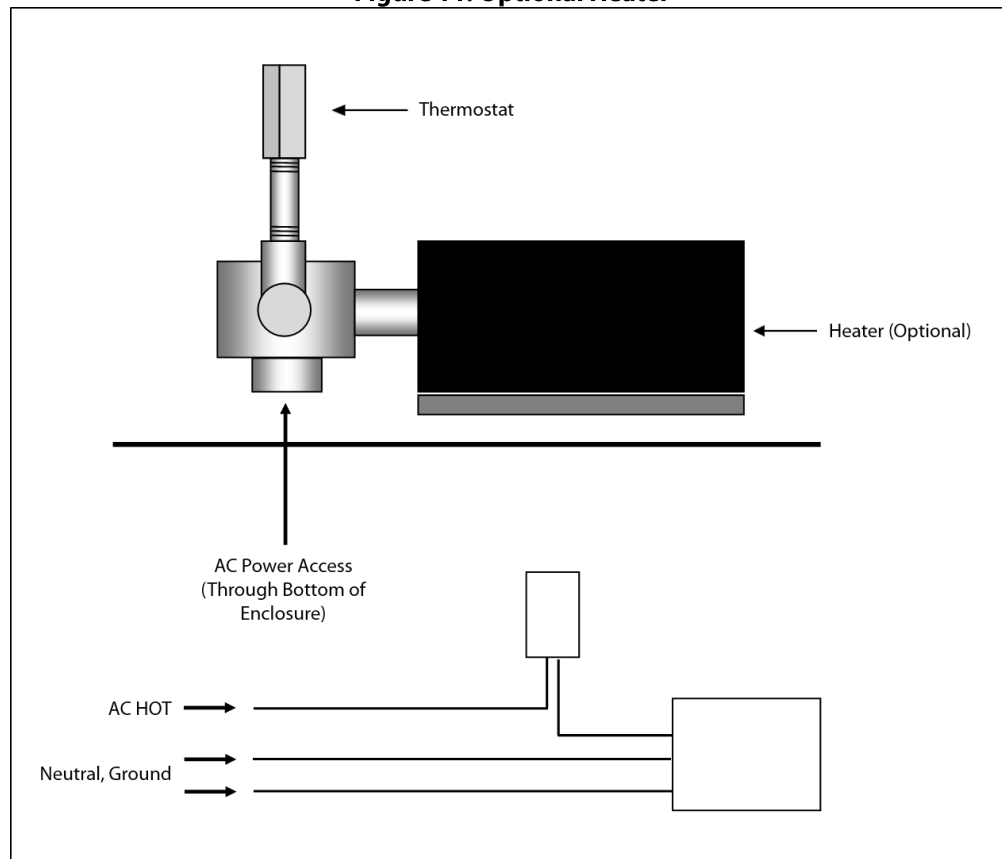
Figure 11: Optional Heater
