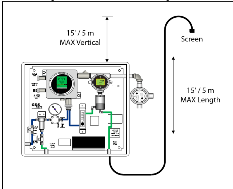
Figure 9: Recommended Exhaust Configuration
