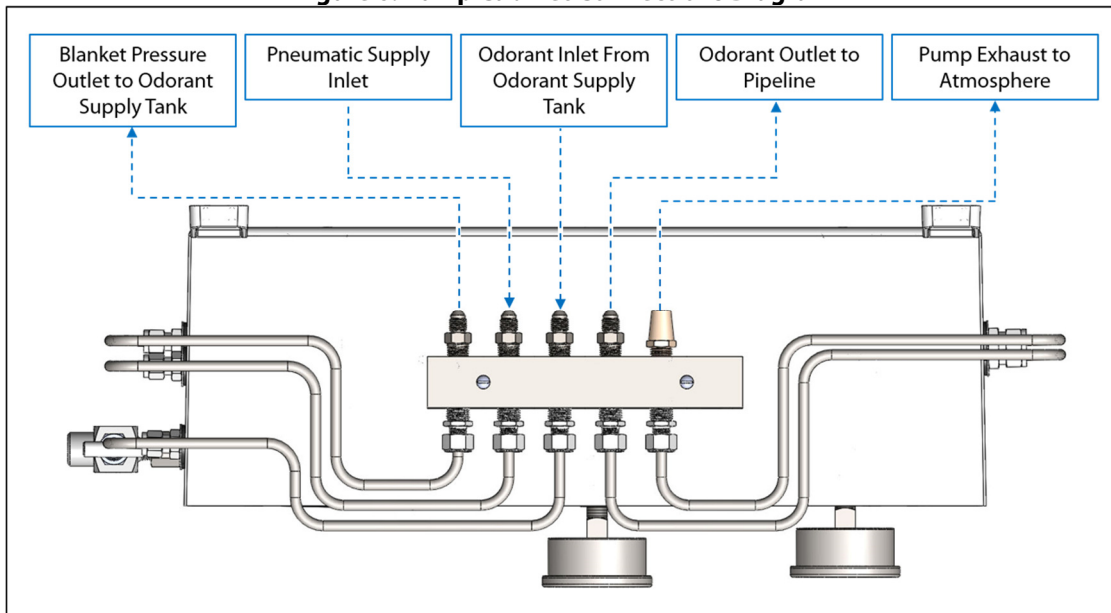
Figure 6: Pump Cabinet Connections Diagram
